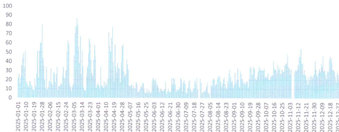
\text{NO}_2 ( \mu\text{g}/\text{m}^3 ) за 24ч "Ватрогаски Дом"
